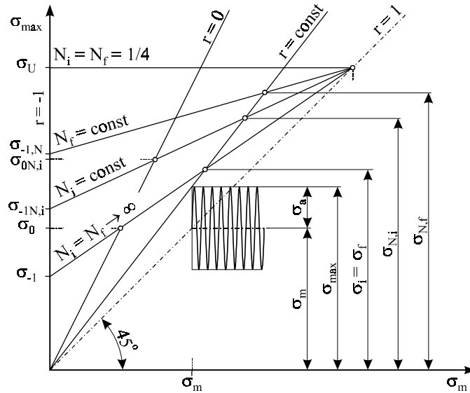
Fig. 3. Crack initiation curves in Smith diagram
