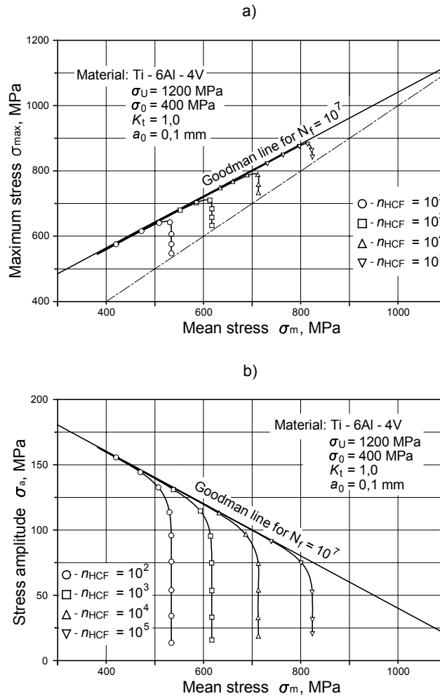
Fig. 5. Fatigue strengths in Smith (a) and Haigh (b) diagram for a combined HCF/LCF loading of a titanium alloy Ti-6Al-4V.
