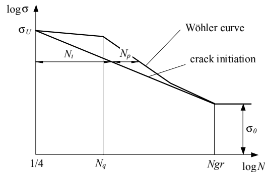
Fig. 2. Approximate design of the CI curve
