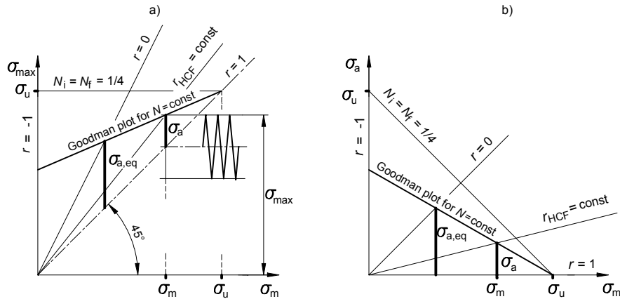
Fig. 4. Reducing the HCF stress amplitude \sigma_a to an equivalent stress amplitude \sigma_{a,eq} at r = 0 in a) Smith diagram, and b) Haigh diagram.
