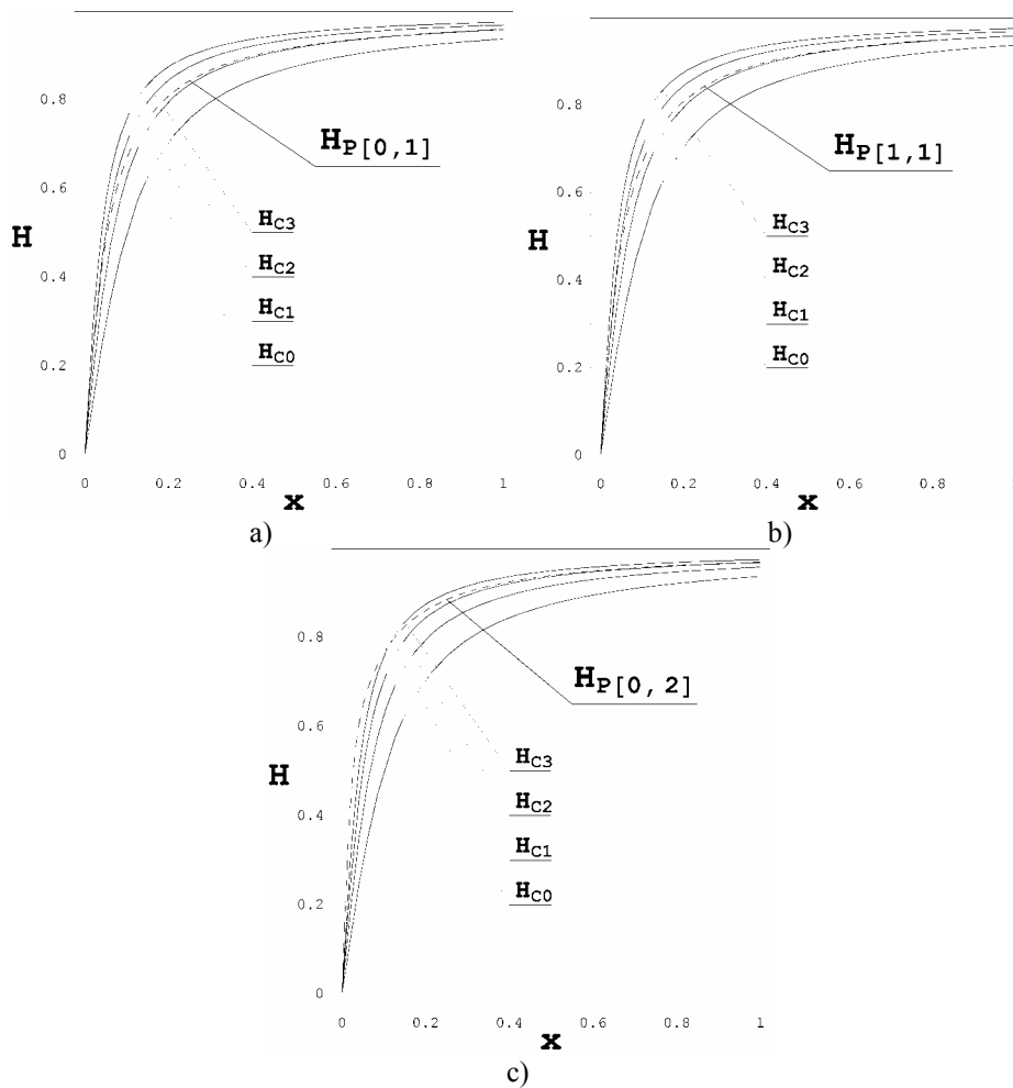
Fig. 1. Normalized inverse tangent function for different values of c ( H_{c0}, H_{c1}, H_{c2}, H_{c3} for c_0 = 10, c_1 = 15, c_2 = 20 and c_3 = 25 ) and Padé approximants H_{P[m,l]} for different m and n values corresponding to (3): (a) m = 0, l = 1 ; (b) m = 1, l = 1 ; (c) m = 0, l = 2
