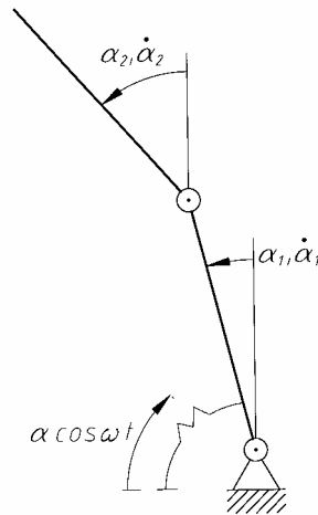
Fig. 2. Mechanical model of a double pendulum
