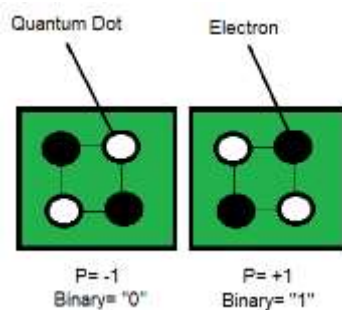
Fig. 1 The polarizations of the QCA cell [9]
