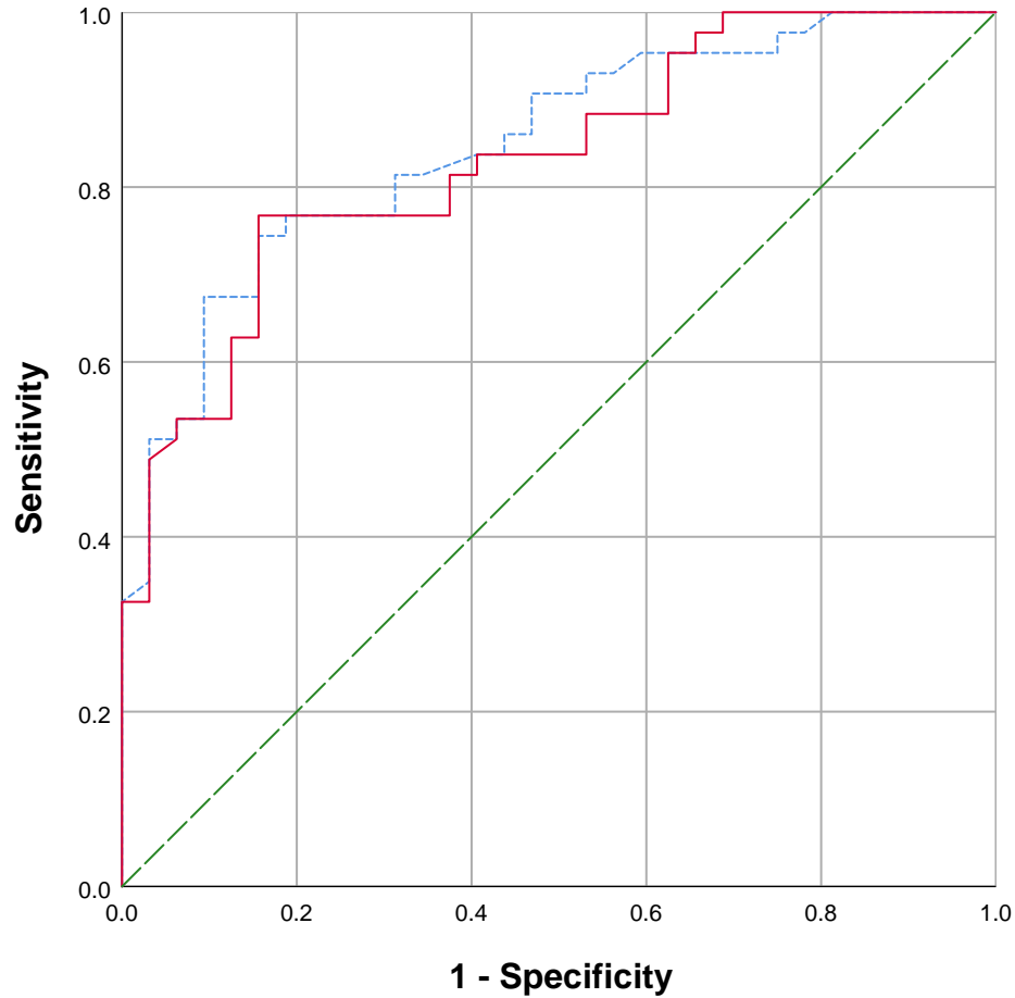
ROC Curve
