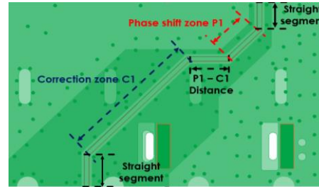
Fig. 18 Optimized Structure
