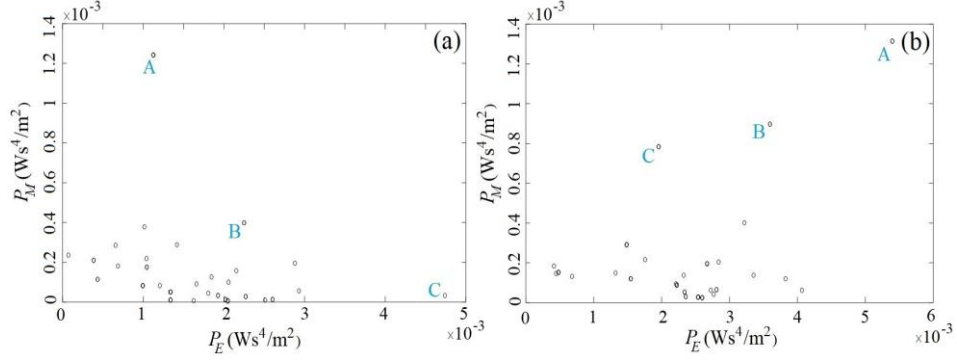
Fig. 4 Multi-objective optimization results and the Pareto front for the first case of optimization case; (a) Series connection, (b) Parallel connection
